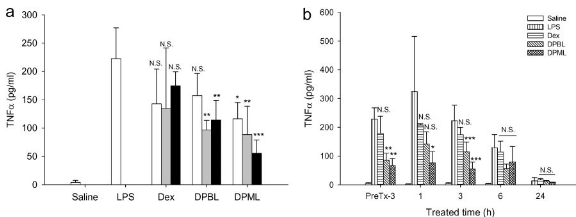
Fig. 4. Dose- (a) and time-response (b) profiles of DPML on the inhibition of \text{TNF}\alpha release after LPS-induced lung inflammation. a, male Wistar rats were administered 0.5 mg/kg i.t. LPS alone or together with free Dex, DPBL, or DPML at a dose of 0.1 (□), 0.25 (▨), and 0.5 (■) mg/kg. The BAL fluid was collected 3 h after challenge. b, male Wistar rats were given drugs at 0.5 mg/kg i.t. together with LPS or pretreated with drugs 1 h before LPS stimulation (pretreatment, PreTx-3), and then the BAL fluid was collected at indicated time or 3 h, respectively. The \text{TNF}\alpha level was measured by ELISA. Results are expressed as mean \pm S.D. of at three experiments. Statistically significant differences (*, P < 0.05 ; **, P < 0.01 ; ***, P < 0.001 ) compared with LPS treatment in each experiment. N.S., not significant.
