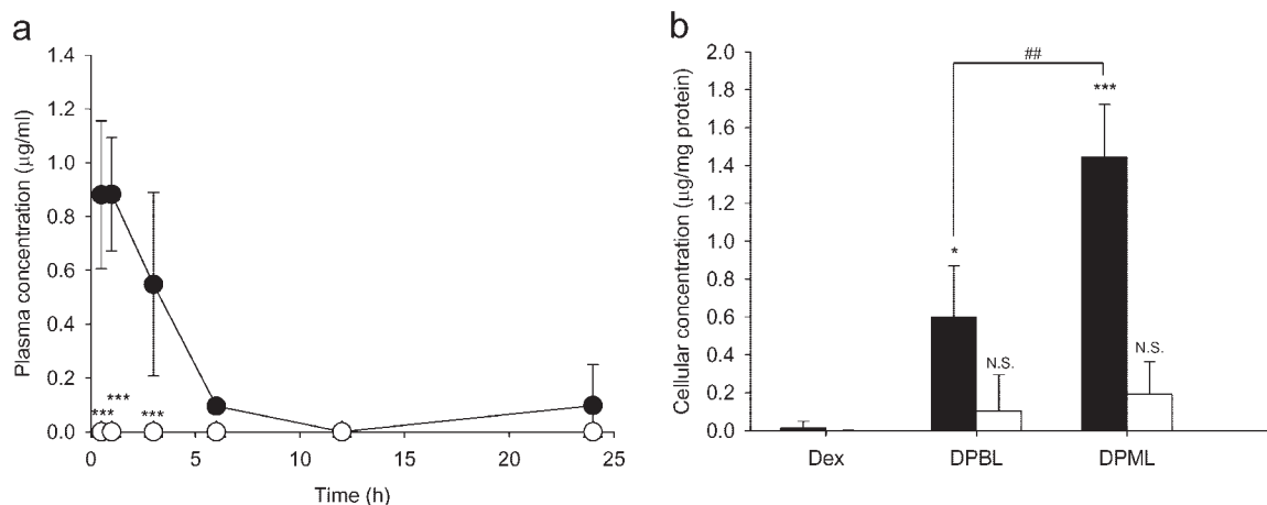
Fig. 1. Biodistribution of liposomal DP and free Dex after intratracheal administration at a dose of 0.5 mg/kg. a, plasma concentration time course of liposomal DP (○) and free Dex (●). b, the concentration of liposomal DP and free Dex in alveolar macrophages at 3 (■) and 24 h (□) post-dosing. Male Wistar rats were intratracheally given liposomal DP and free Dex at 0.5 mg/kg, and then plasma and alveolar macrophages were collected at indicated time points (0.5–24 h). The concentration of drugs was determined by HPLC systems. Results are expressed as mean \pm S.D. of three experiments. Statistically significant differences (*, P < 0.05 ; ***, P < 0.001 ) compared with Dex treatment in each experiment (##, P < 0.01 ) with each pair of treatments. N.S., not significant.
