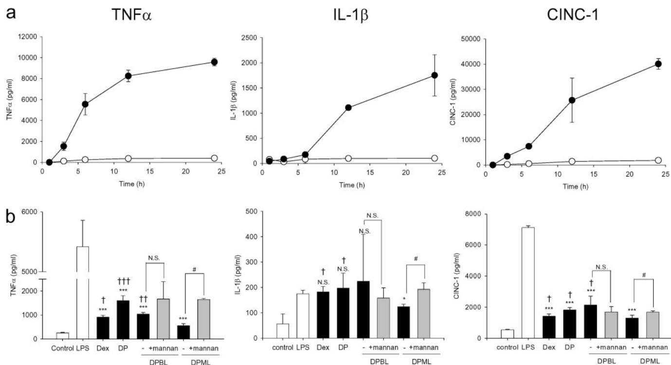
Fig. 2. Effects of DPML on inhibition of LPS-induced cytokine and chemokine release in vitro. a, time course of TNF \alpha , IL-1 \beta , and CINC-1 protein levels after LPS stimulation at 1 \mu g/ml (●) and control (○). b, inhibition of TNF \alpha , IL-1 \beta , and CINC-1 protein levels after treatment. The alveolar macrophages were incubated with 1 \mu g/ml LPS alone or coincubated with 0.1 \mu M free drugs (Dex or DP) or liposomal DP (■). For the uptake inhibition, mannan was also coincubated at 1 mg/ml (□). The cytokine and chemokine levels in the supernatant were determined by ELISA after a 6-h incubation. Results are expressed as mean \pm S.D. of at least three experiments. Statistically significant differences (*, P < 0.05 ; ***, P < 0.001 ) compared with LPS treatment in each experiment (†, P < 0.05 ; ††, P < 0.01 ; †††, P < 0.001 ) with DPML treatments (#, P < 0.05 ) with each pair of treatments. N.S., not significant.
