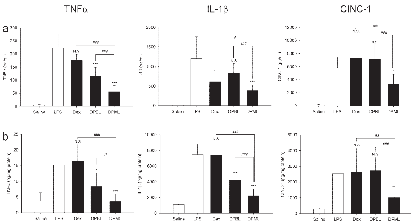
Fig. 5. Efficient inhibition of cytokine release after intratracheal instillation of DPML in BAL fluid (a) and lung tissue (b). Male Wistar rats were administered 0.5 mg/kg i.t. LPS alone ( \square ) or together with free Dex, DPBL, or DPML ( \blacksquare ) at a dose of 0.5 mg/kg. The BAL fluid and lung tissue were collected 3 h after challenge, and cytokine levels were measured by ELISA. Results are expressed as a mean \pm S.D. of at least six experiments. Statistically significant differences (*, P < 0.05 ; **, P < 0.01 ; ***, P < 0.001 ) compared with LPS treatment in each experiment (#, P < 0.05 ; ##, P < 0.01 ; ###, P < 0.001 ) with each pair of treatments. N.S., not significant.
